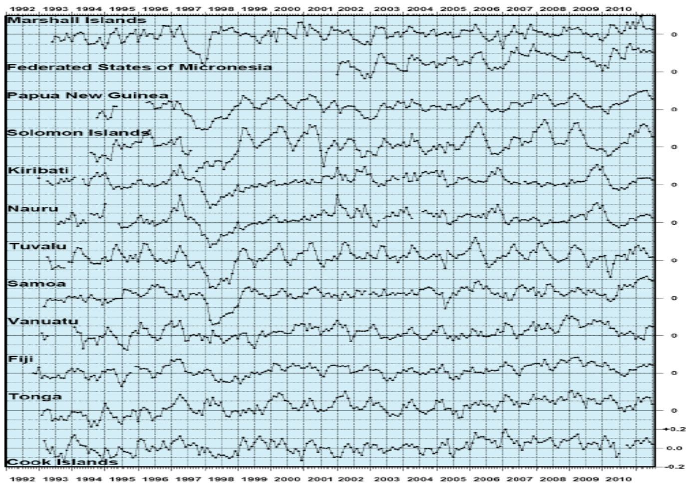
Figure 10. Monthly mean sea levels to June 2011.
