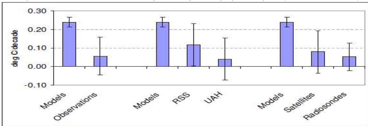
Figure 3: Modeled and estimated trends (1979-2009, C decade -1 ) in the tropics, mid-troposphere (MT) layer
