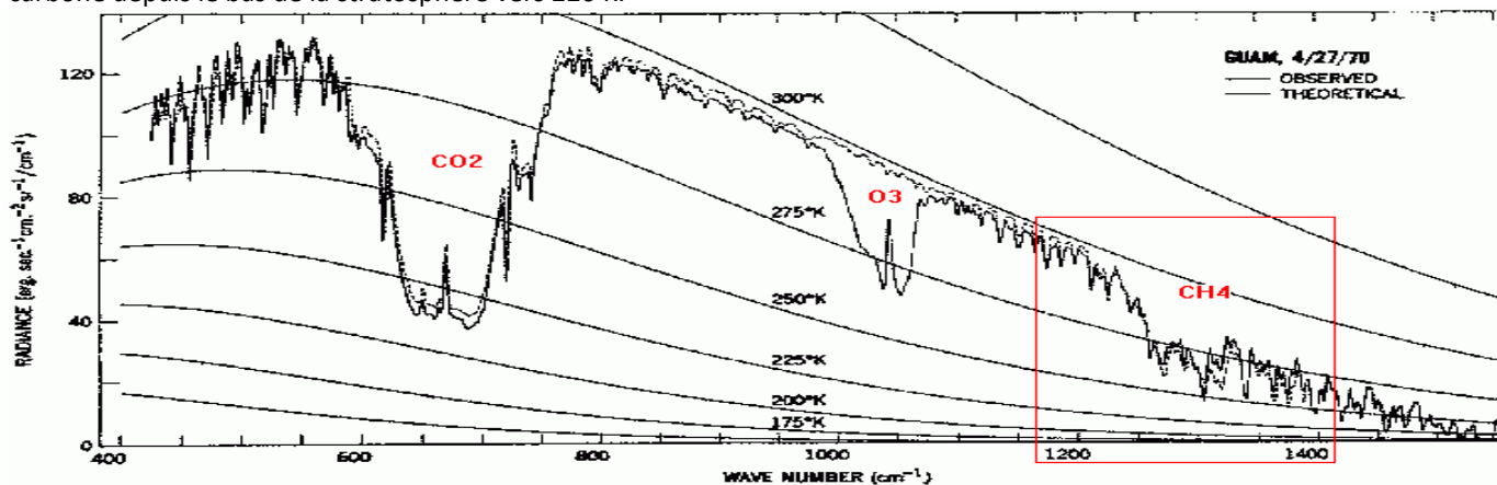
Fig. 3. Comparison of observed and theoretical radiances for a clear atmosphere near Guam at 15.1°N and 215.3°W on April 27, 1970.
