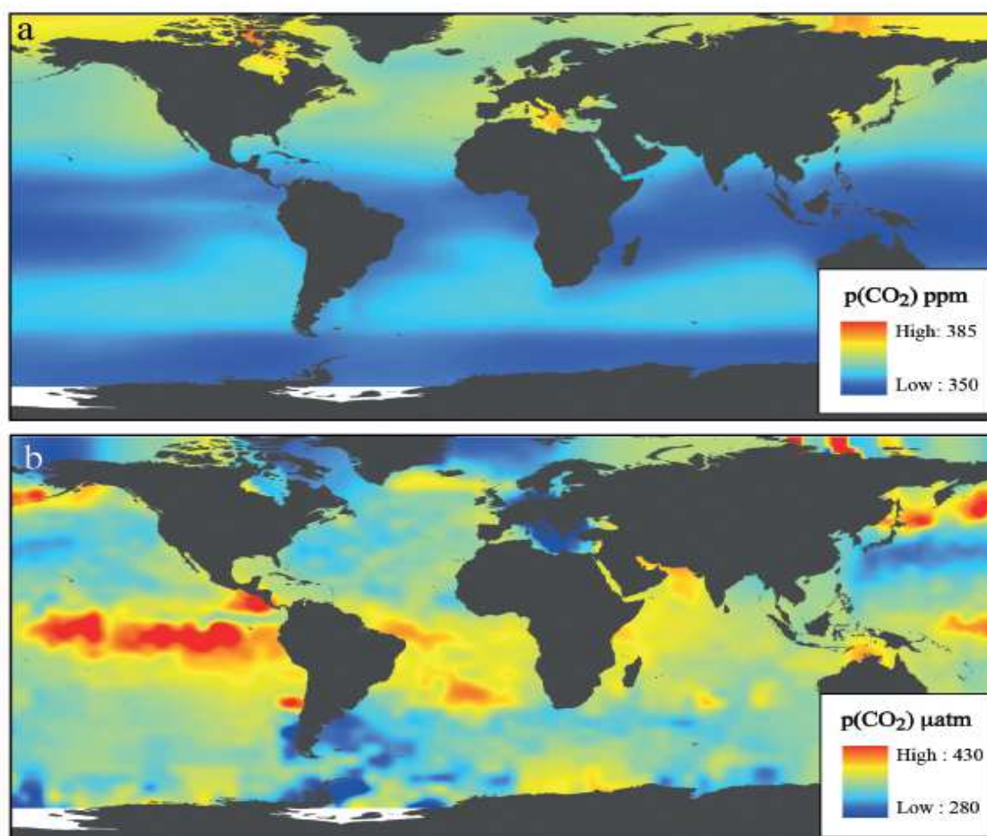
Figure 3.1 Carbon dioxide concentrations over the ocean. A. Atmospheric p(CO 2 ) levels (ppm). B. Surface p(CO 2 ) (μatm). Note the change in scale among plots. Data from Takahashi et al. (2009).
